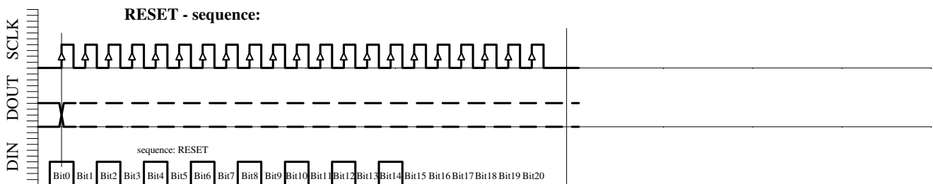
Fig. 6e: RESET sequence (21 bit)
